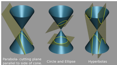
Circle and Ellipse
